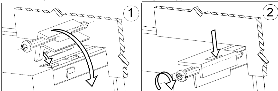
Fig.2. Meter fixing
